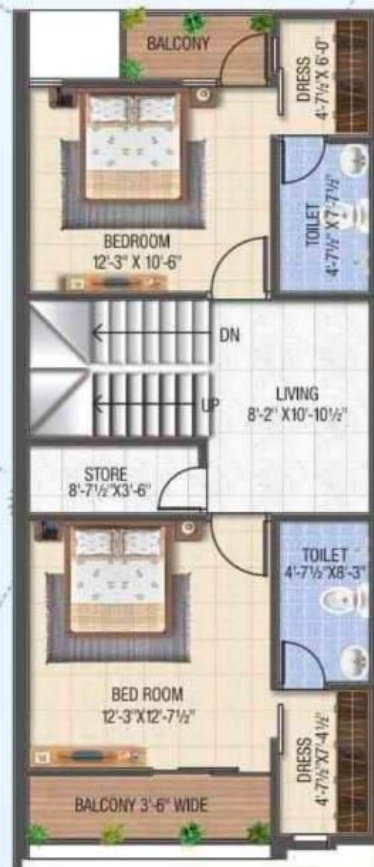
LIG WEST FACING FIRST FLOOR PLAN Plot Size : 18' x 44'
