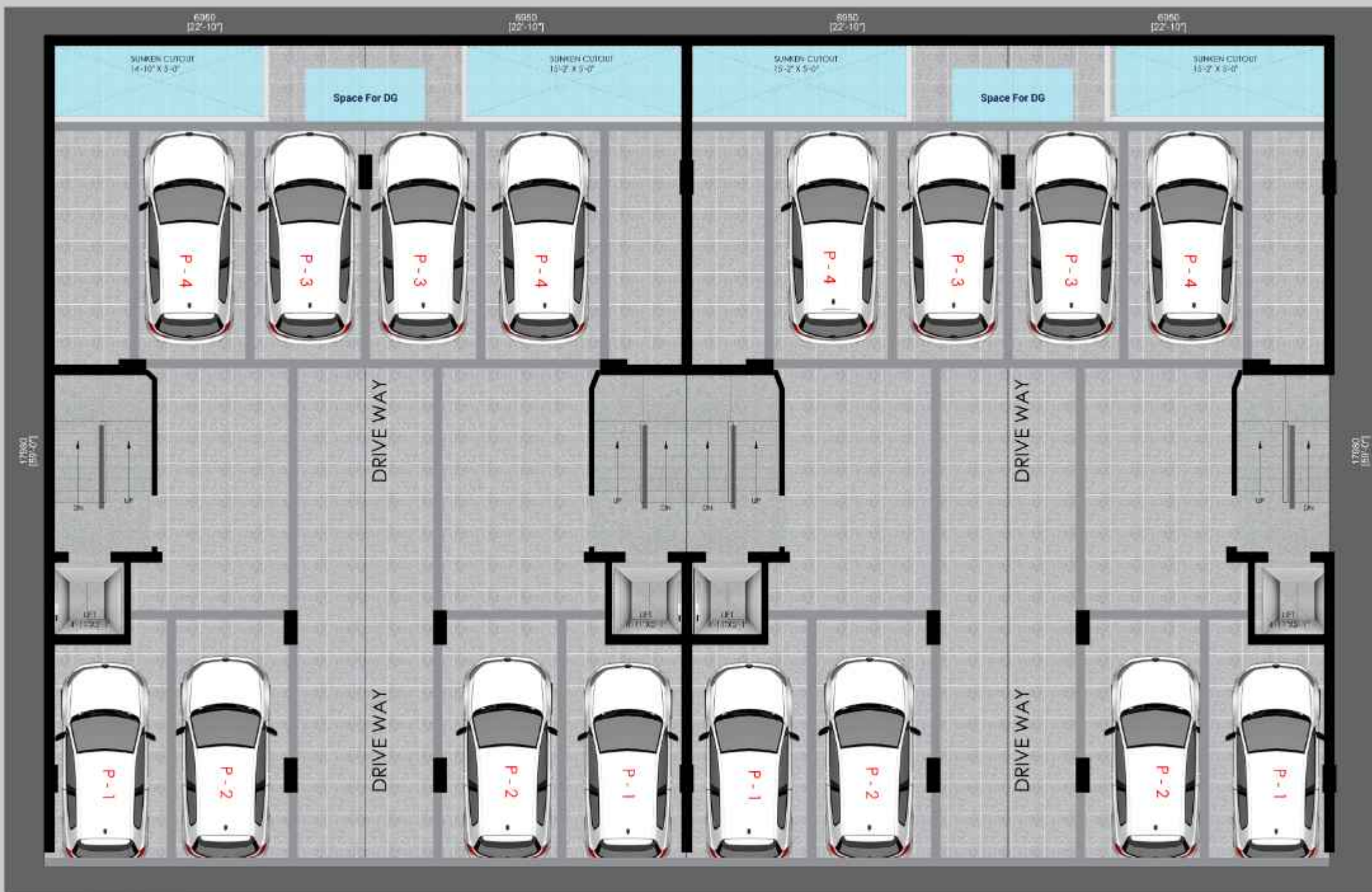
STILT PLAN
